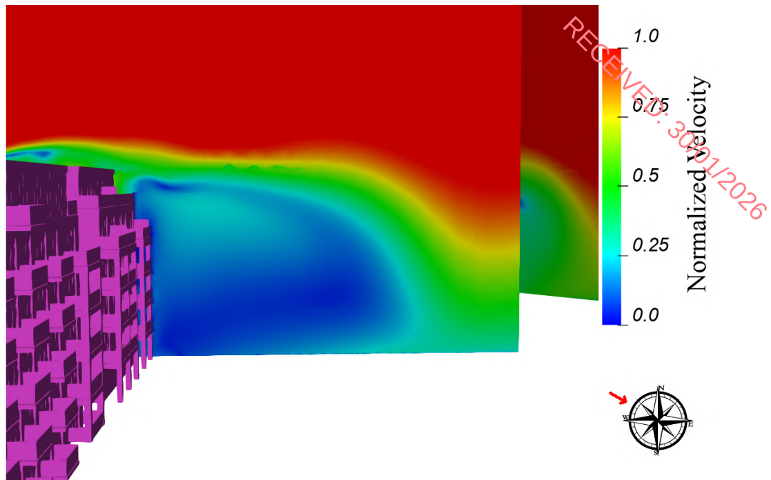
Figure 12.62.: Example of wind results on Balconies of E1- Flow Velocity Results - Wind Direction: 300°
