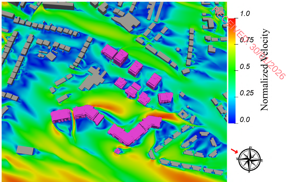
Figure 12.47: Flow Velocity Results at Z=1.8\text{m} above the ground Wind Direction: West-North-West
