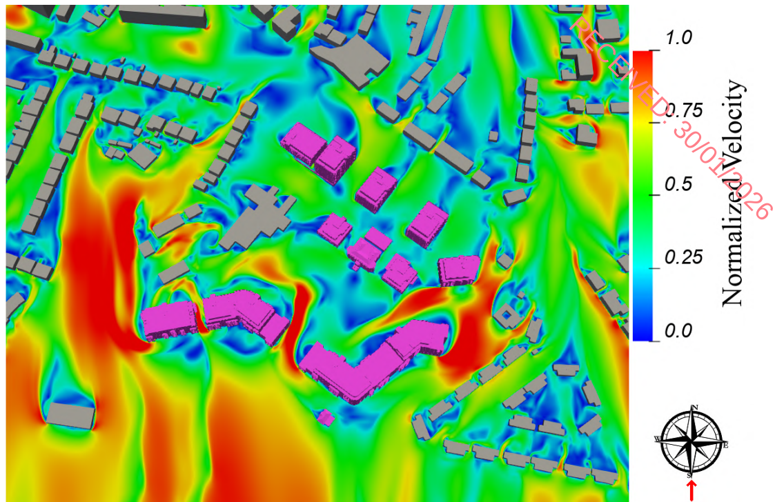
Figure 12.43: Flow Velocity Results at Z=1.8m above the ground Wind Direction: South
