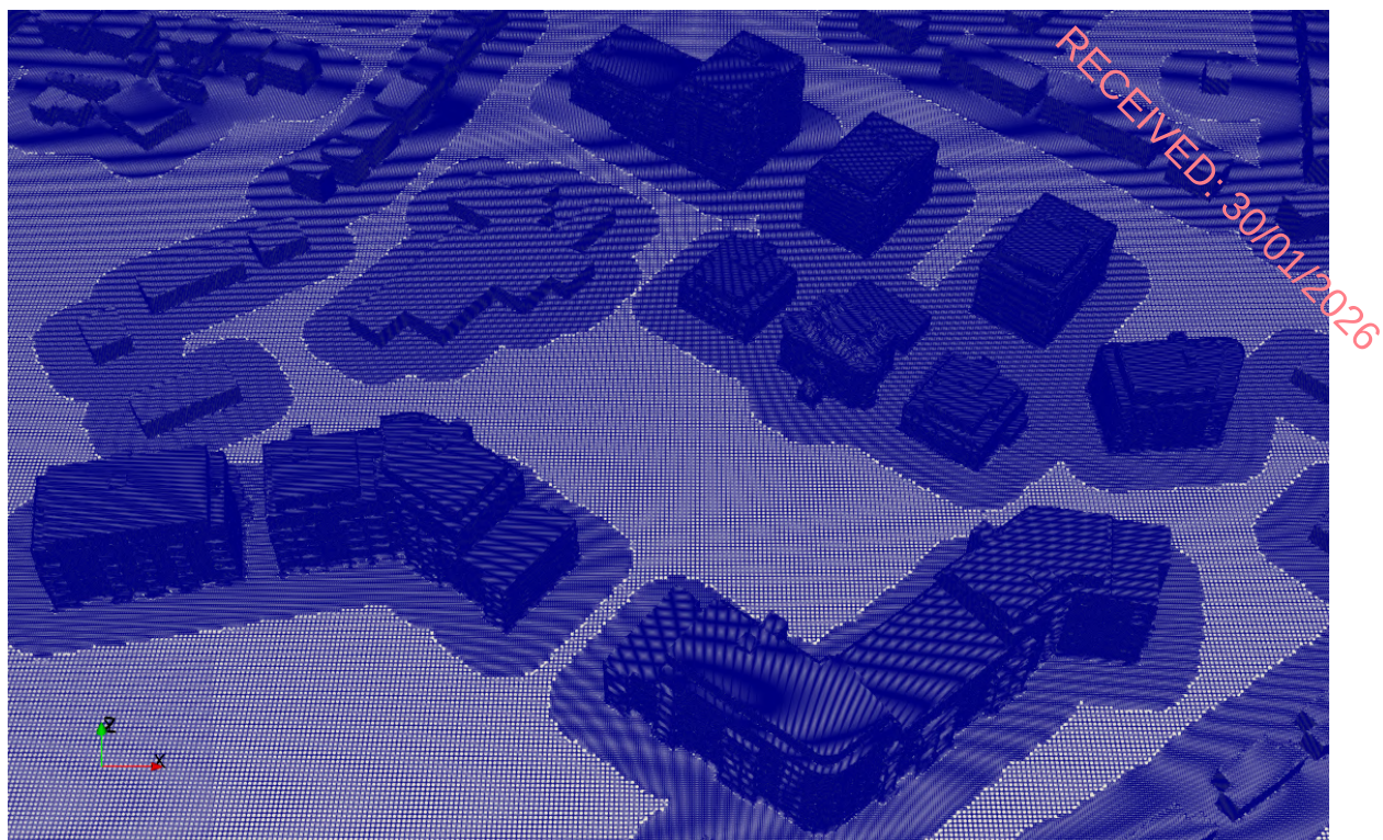
Figure 32.12 Computational Mesh of Proposed Development:
