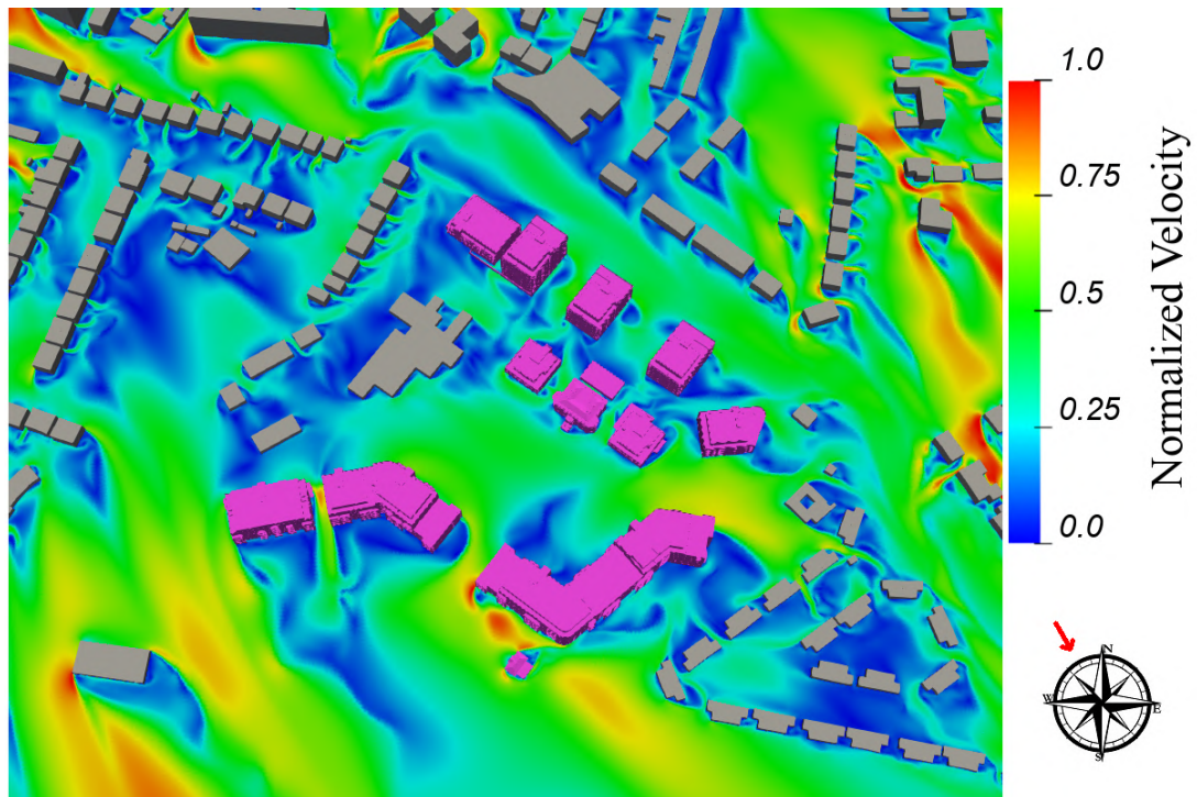
Figure 12.48: Flow Velocity Results at Z=1.8\text{m} above the ground Wind Direction: North-West
