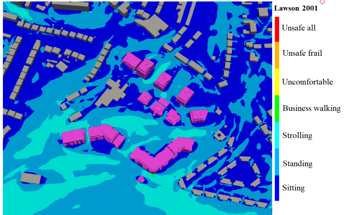
Figure 12.49: Ground Floor - Lawson Discomfort Map - 3D View.
